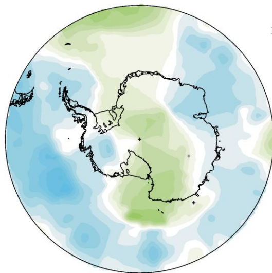
Air temperature 201012 versus average 1998-2006
