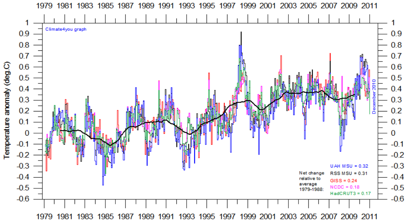
6 Superimposed plot of all five global monthly temperature estimates shown above. As the base period differs for the different temperature estimates, they have all been normalised by comparing to the average value of their initial 120 months (10 years) from January 1979 to December 1988. The heavy black line represents the simple running 37 month (c. 3 year) mean of the average of all five temperature records. The numbers shown in the lower right corner represent the temperature anomaly relative to the above average.
