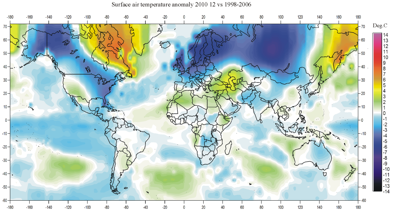
Air temperature 201012 versus average 1998-2006
