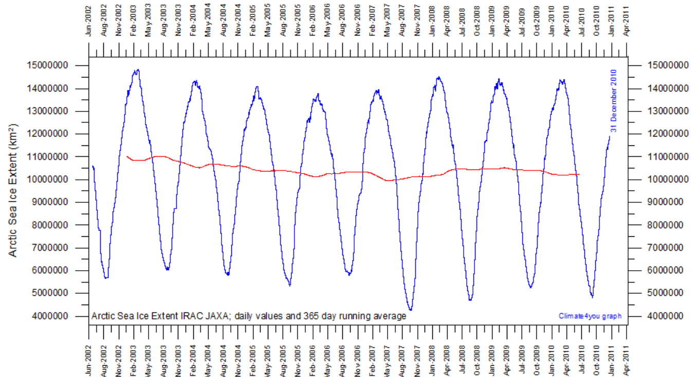
Graph showing daily Arctic sea ice extent since June 2002, to 31/12 2010, by courtesy of Japan Aerospace Exploration Agency (JAXA) .
